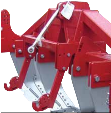
3-point linkage for PTO implement.
